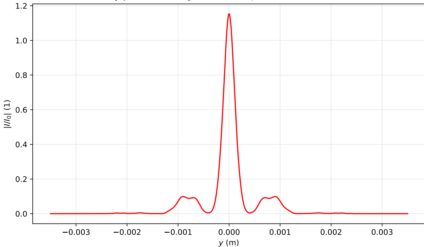
Intensity profile I(x=0, y, z=1.672)/I_0 , \text{Pin}=8.5\text{Pcr} , artificial time
